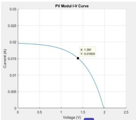
Figure 8. PV Modul I-V Curve
