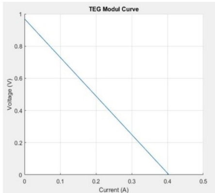
Figure 10. TEG Modul I-V Curve
