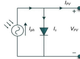
Figure 2. PV cell circuit model ideal
