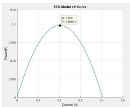
Figure 11. TEG Modul I-P Curve
