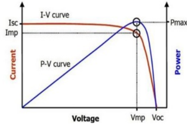
Figure 4. PV curve : I-V (red) dan P-V(blue) curve [17]
