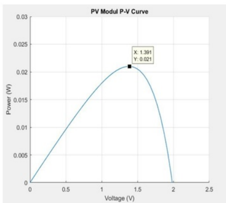
Figure 9. PV Modul P-V Curve
