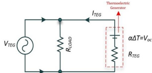
Figure 5. TEG circuit model
