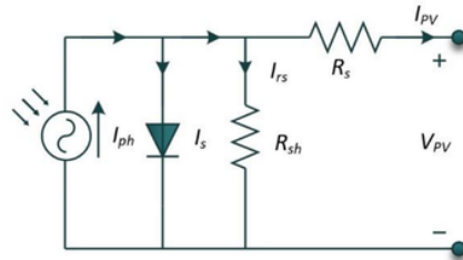
Figure 3. PV cell circuit model in one diode
