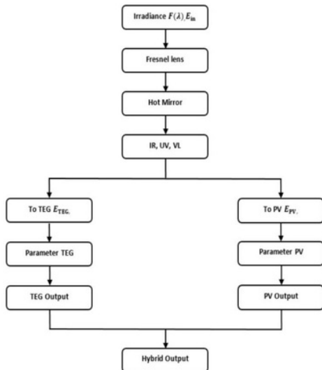
Figure 6. Schematic Calculation of PV-TEG hybrids
